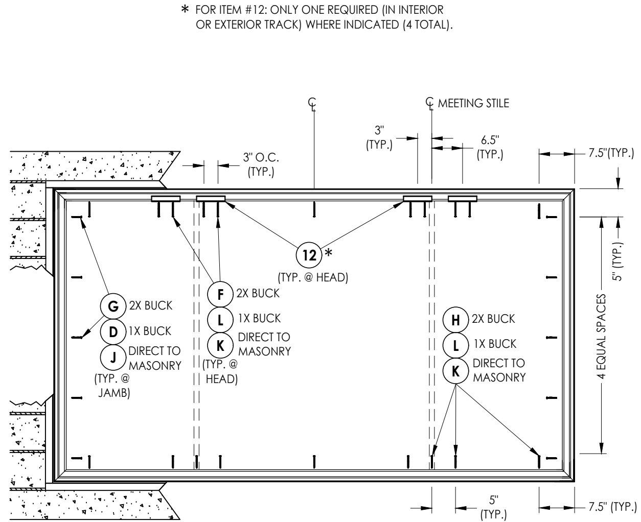
FRAME ANCHORING
